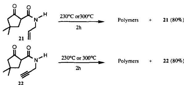
Scheme I: Thermolysis of N -unsaturated alkyl- \beta -ketoamides
